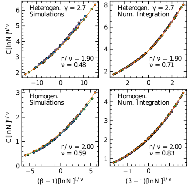
Fig. 1. Data collapse based on the finite size scaling ansatz C(\beta, N) = [\ln N]^{-\frac{\eta}{\nu}} f((\beta - \beta_c) [\ln N]^{\frac{1}{\nu}}) for heterogeneous networks with \gamma = 2.7 (top row) and homogeneous networks (bottom row). Left column correspond to numerical simulations with sizes in the range N \in (5 \times 10^2, 10^5) , whereas the right column is obtained from numerical integration in the range N \in (5 \times 10^5, 10^8) .
